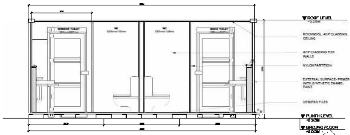
Proposed container toilet section
